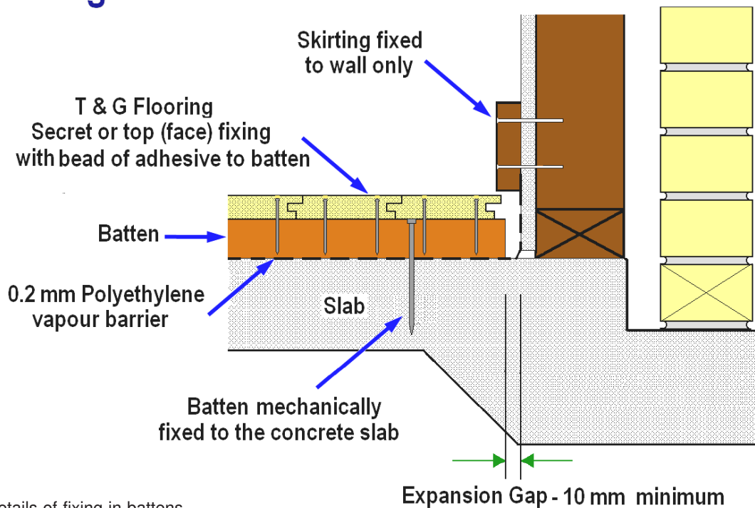
Figure 4 - Details of fixing in battens
