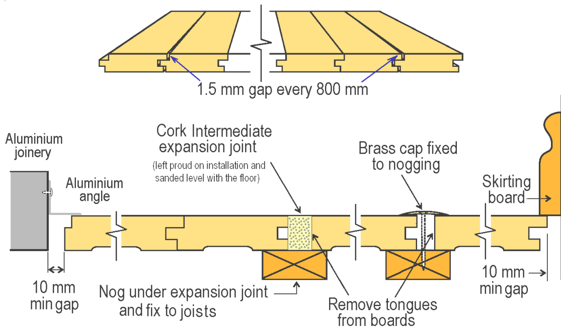
Figure 2 - Expansion Gap details
