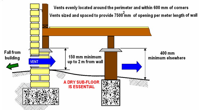
Figure 1 - Sub-floor Ventilation
